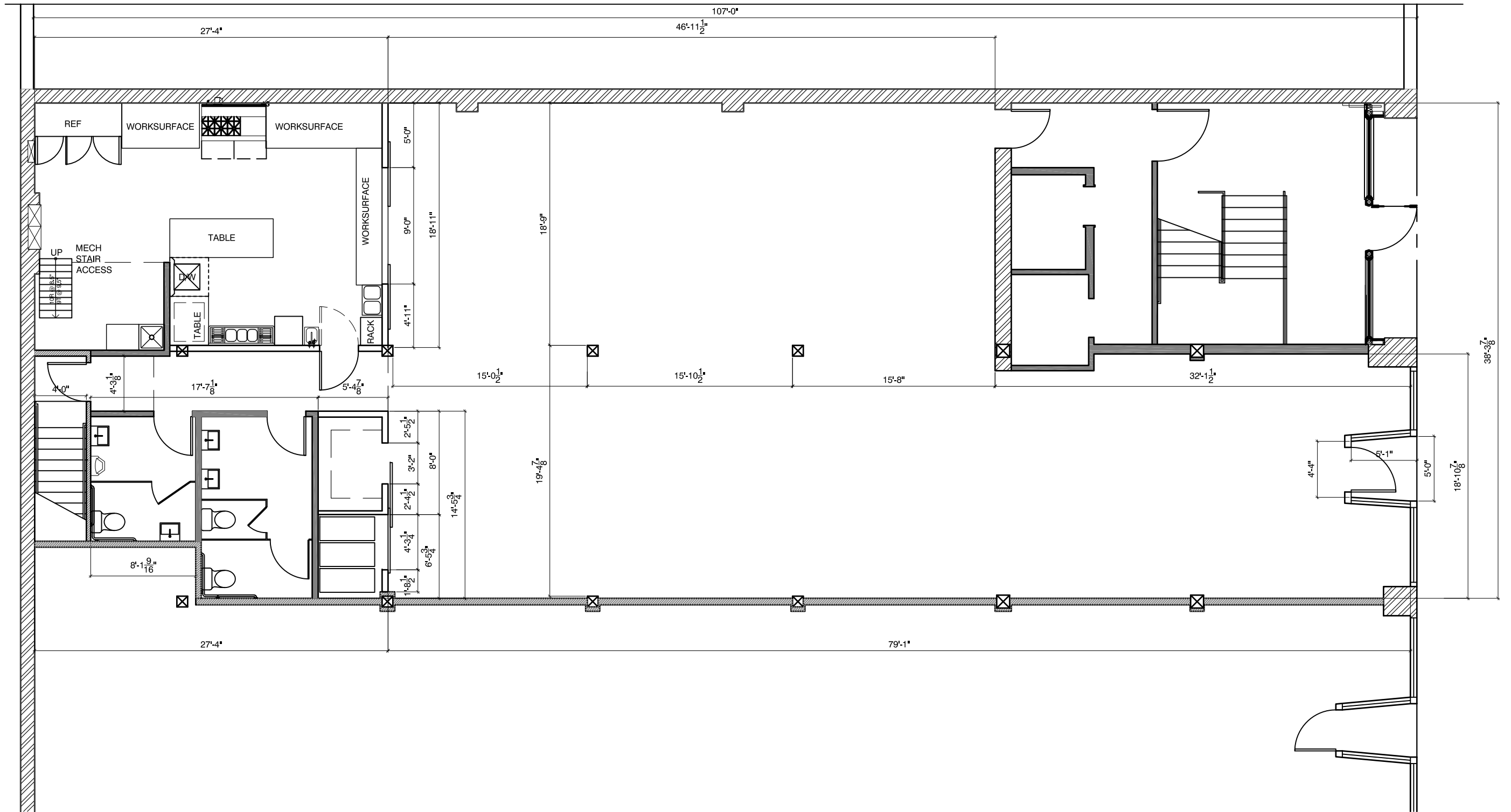
1 FLOOR PLAN 1/8" = 1'-0"
